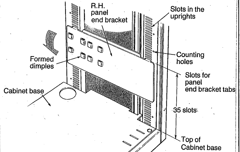
Figure 1. Divider kit locating, above the cabinet base
