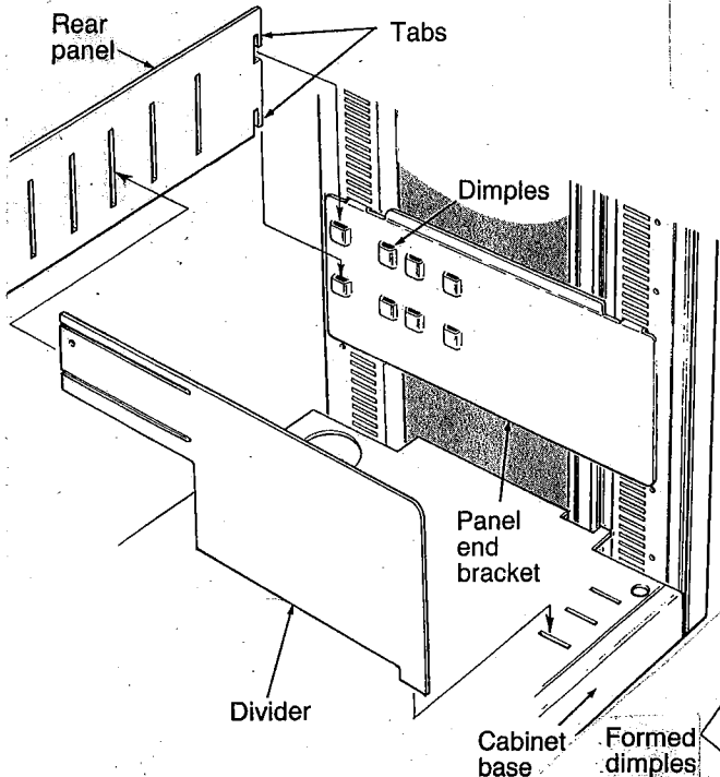
Figure 3. Rear panel installation
