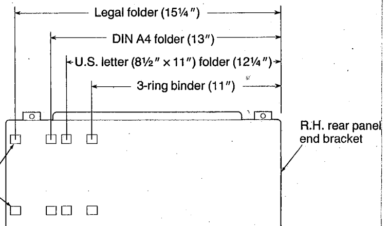
Figure 4. Rear panel positions
