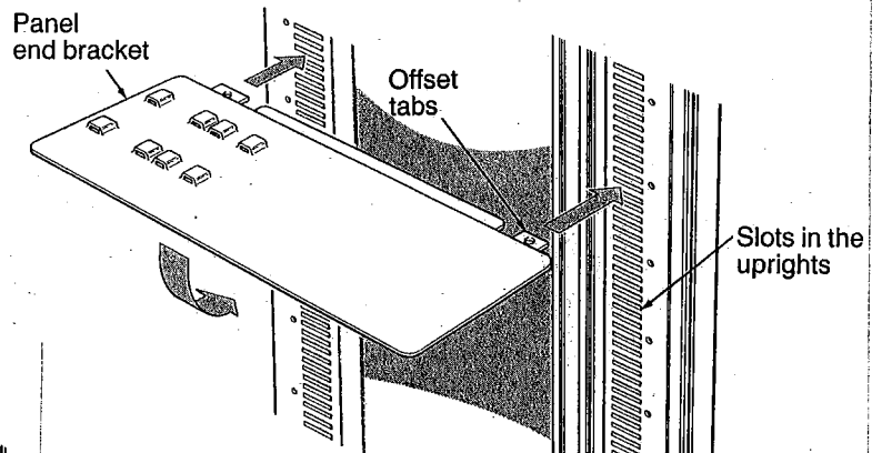
Figure 2. Panel end bracket installation
